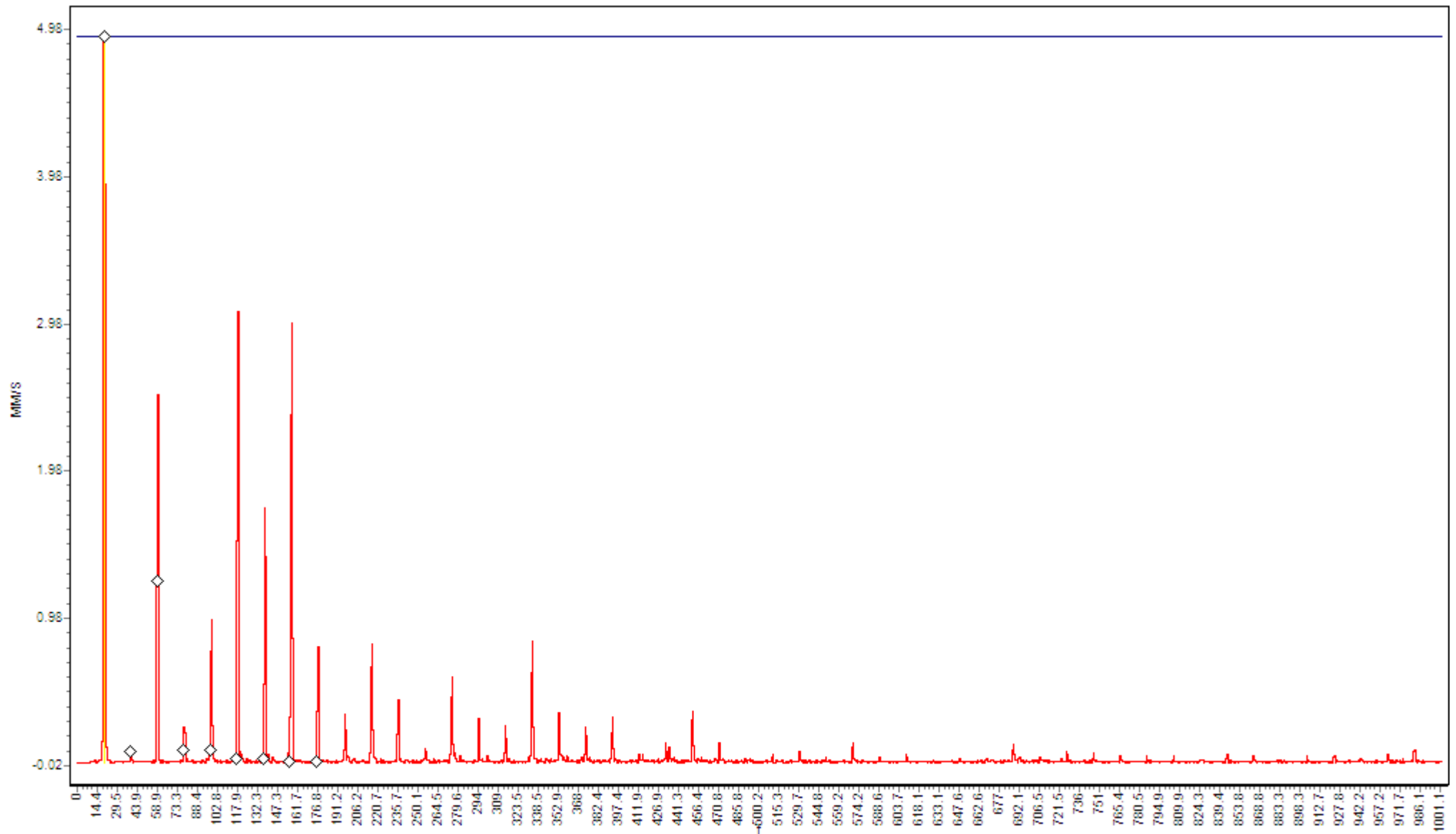
Metzin/Waterfall FFT/Brg Good &Bad/Unbal compare (2009/02/16 11:57:16 - FFT Lin (1600) A)
