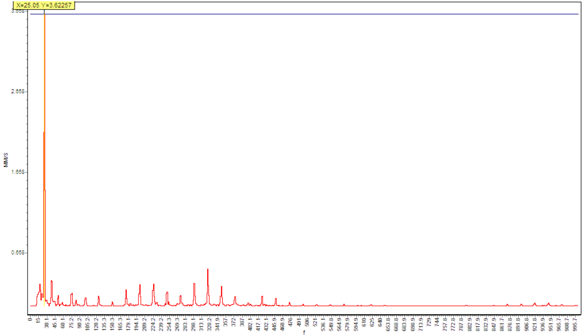
SI Group/Process Area/Reactor_R1/R1-10_2DEH (0917_120508 - FFT Lin (800)) Rms value 4.64mm/s; non std flex foundation equipment required data trend monitoring.
